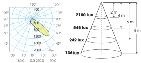
HBM03 200W
