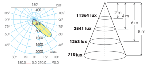
HBM03 400W
